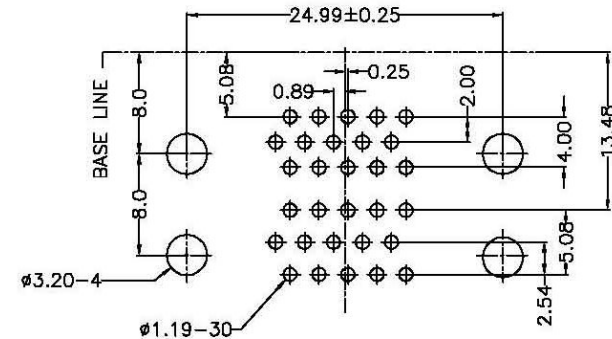
RECOMMEND P.C.B. LAYOUT BOTTOM VIEW
